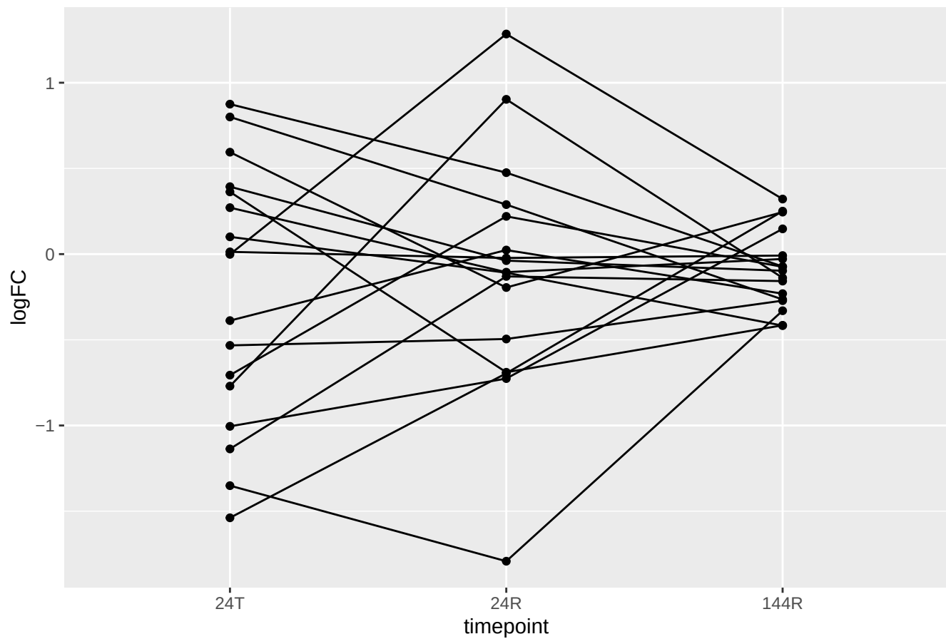
LFC at timepoints of genes switched on MER61E TE
